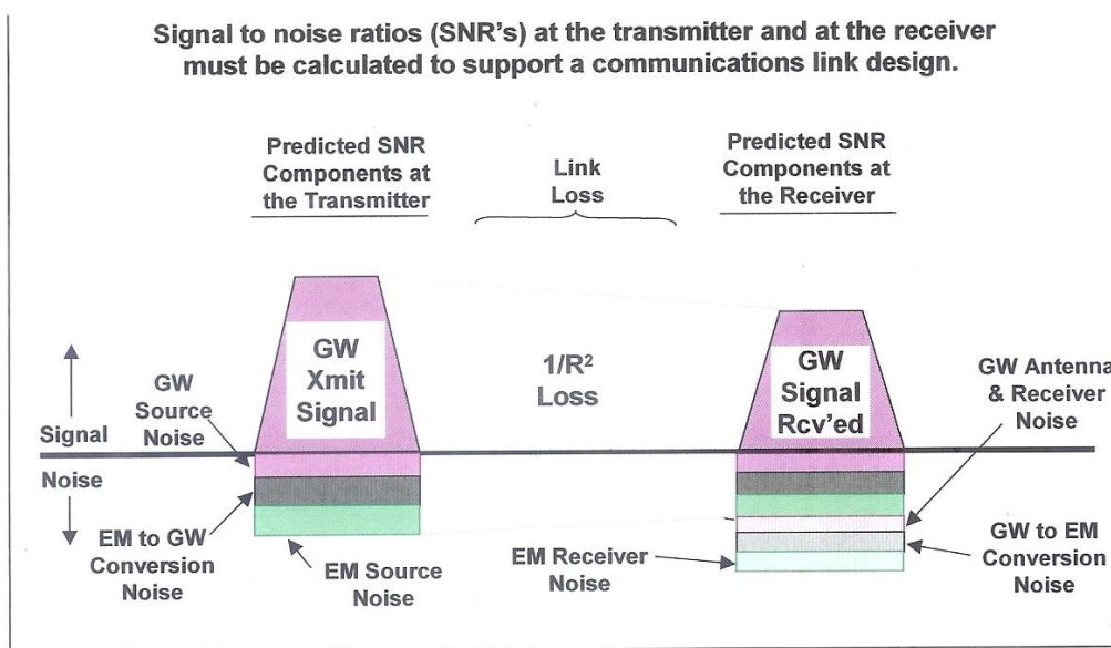
Figure 3.1a. Conceptual SNR Fill Factors: Signal and Noise Components
