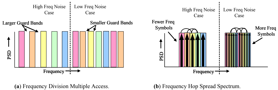
Figure 3.2c. The Impact of Frequency Noise Improvements on FDMA and FHSS.
