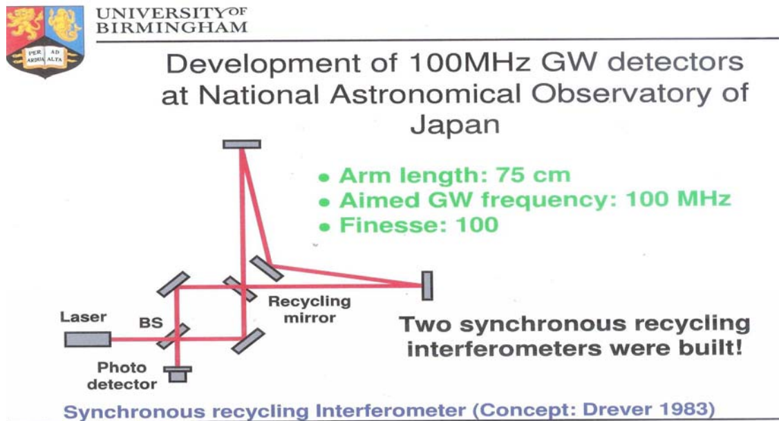
Figure 2.2.1c. The National Astronomical Observatory of Japan 100MHz Detector. Cruise (2008).
