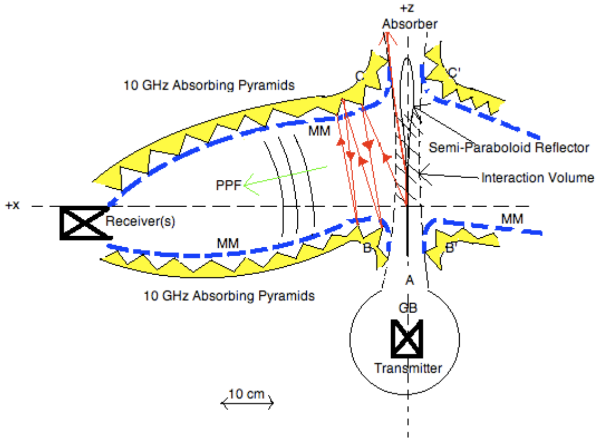
Figure 2.2.4b Side-view Schematic of the Li-Baker HFGW Detector Exhibiting Microwave Absorbent Walls.
